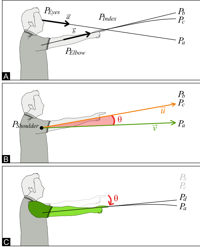
Figure 2: Warping Deixis uses A) a Bayesian model to predict the referent's location interpreted by the observer, P_c , and B) calculates the necessary arm displacement to a C) distal location P_d such that extrapolations would result in their correctly interpreting the pointer's intended target P_a .
